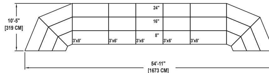
WINGED SHAPE
