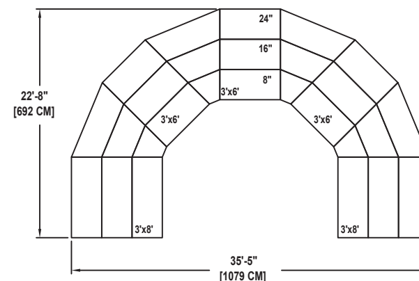
SEMICIRCLE SHAPE
