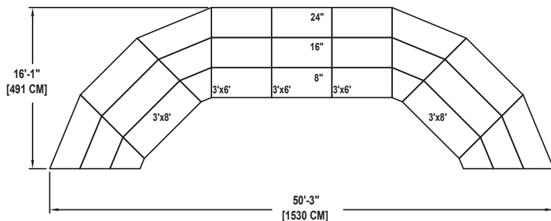
ARC SHAPE
